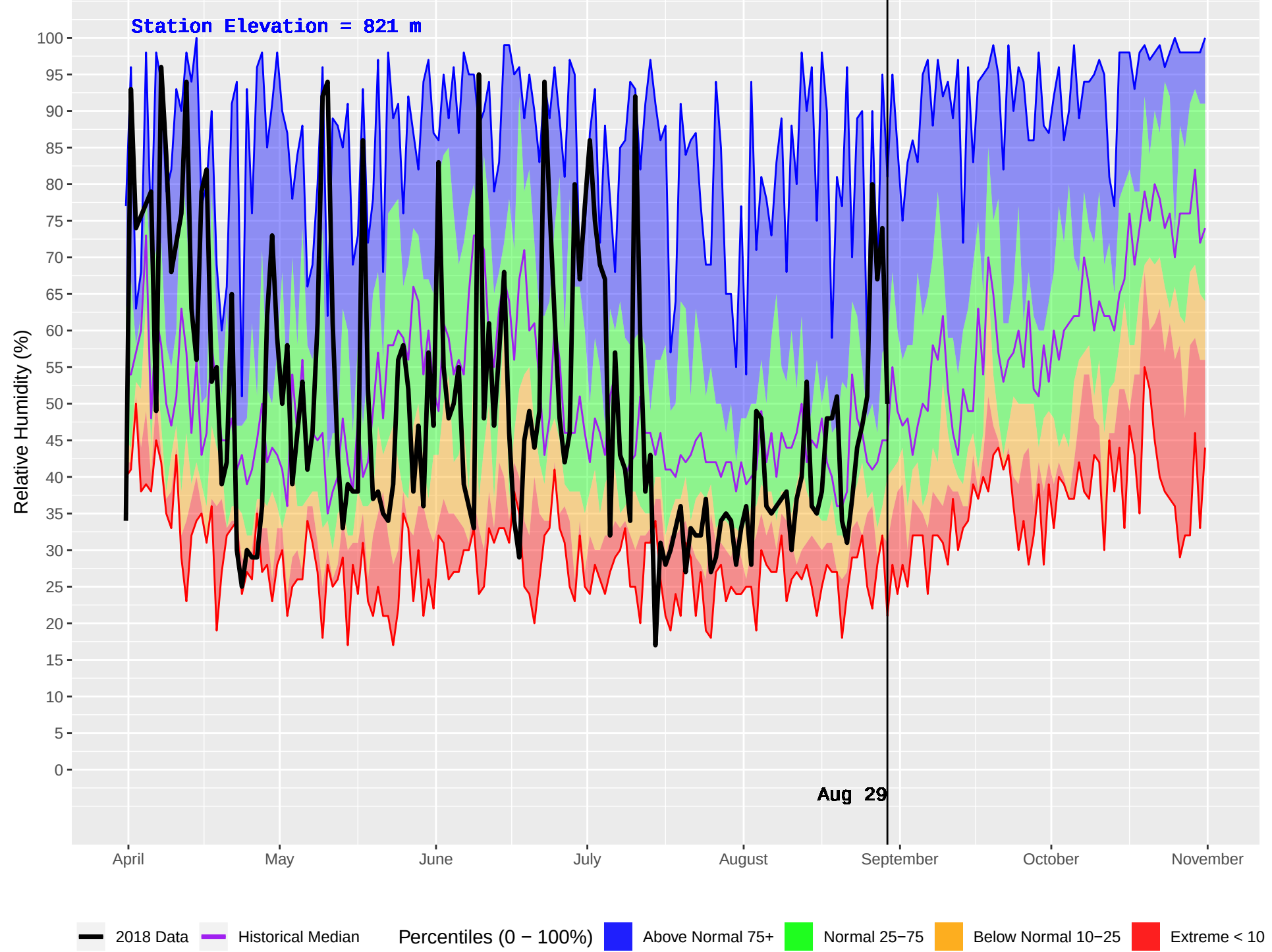
AKOKLI CREEK (838) : Historical (2003–2016) and Current (2018) Daily Relative Humidity
