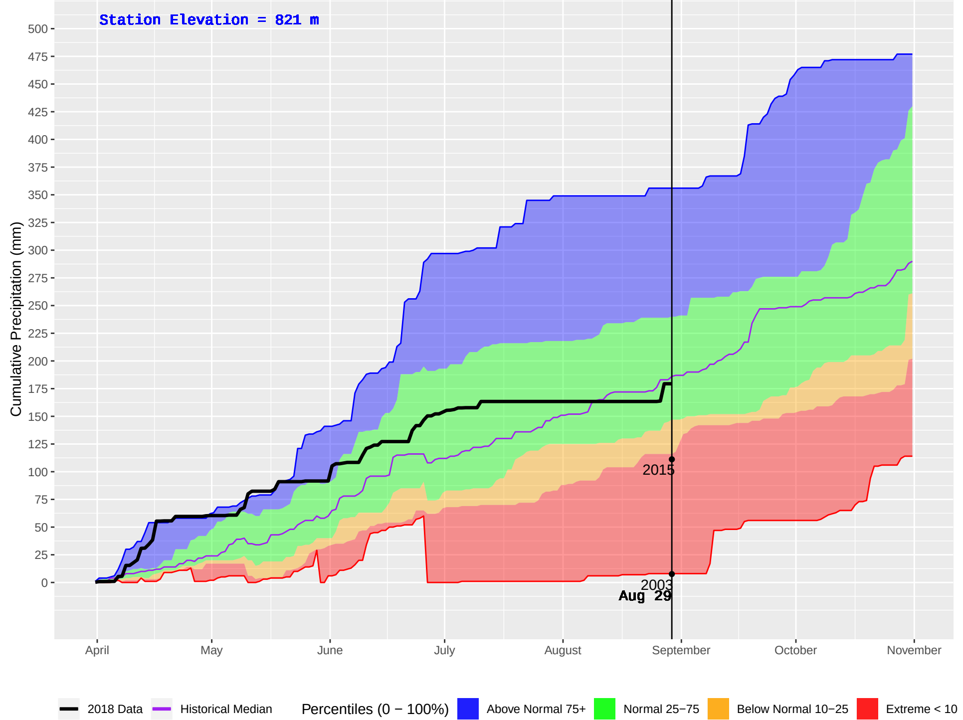
AKOKLI CREEK (838) : Historical (2003–2016) and Current (2018) Daily Cumulative Precipitation
