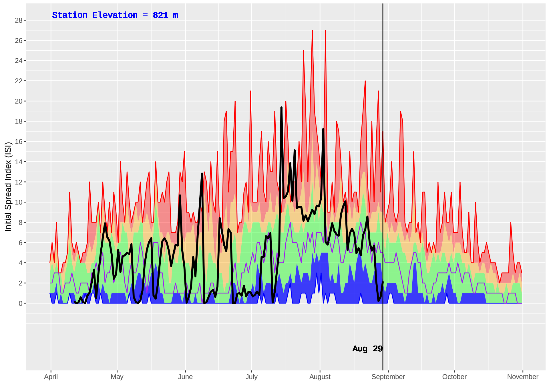
AKOKLI CREEK (838) : Historical (2003–2016) and Current (2018) Daily Initial Spread Index (ISI)
