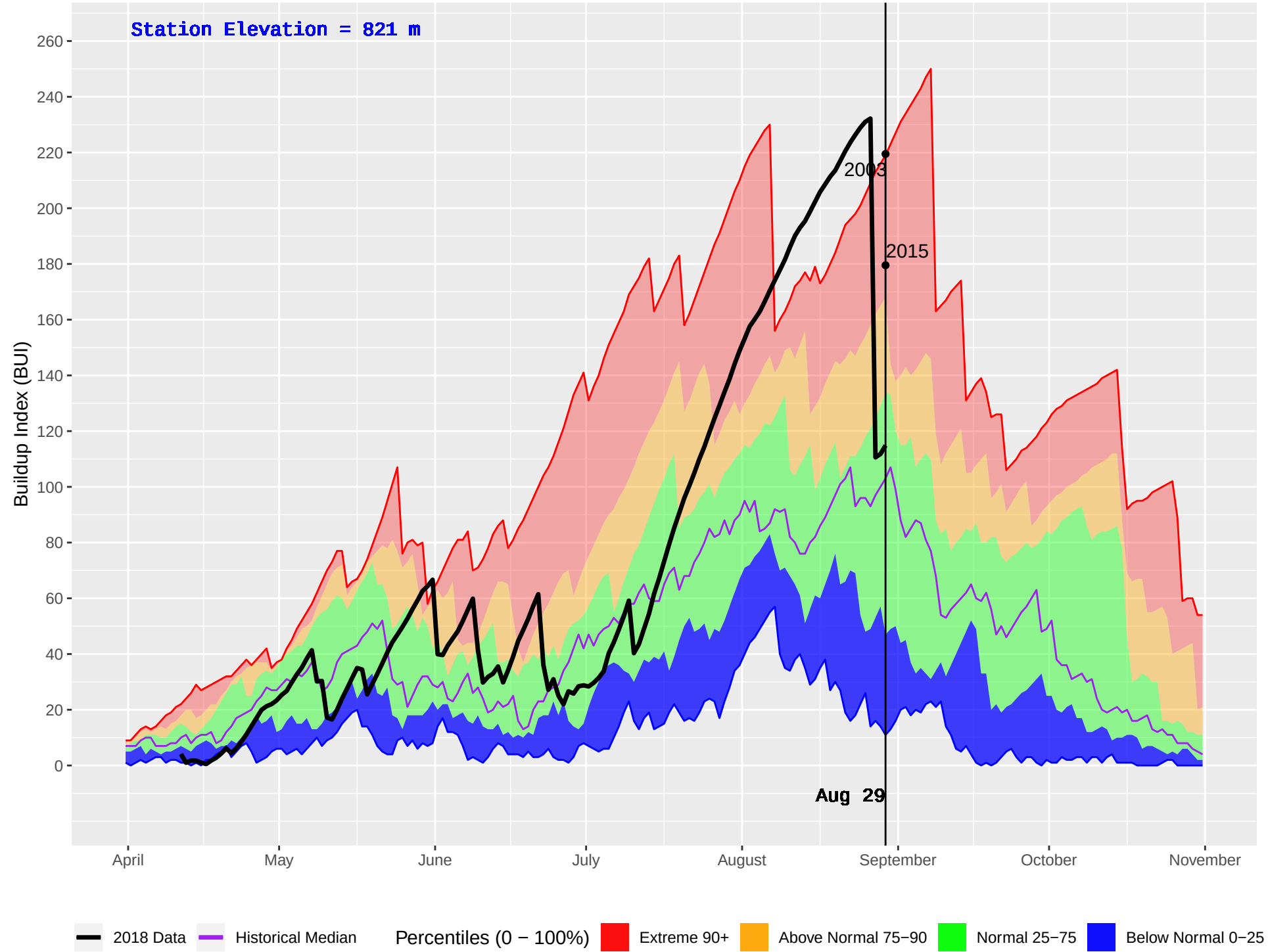
AKOKLI CREEK (838) : Historical (2003–2016) and Current (2018) Daily Buildup Index (BUI)
