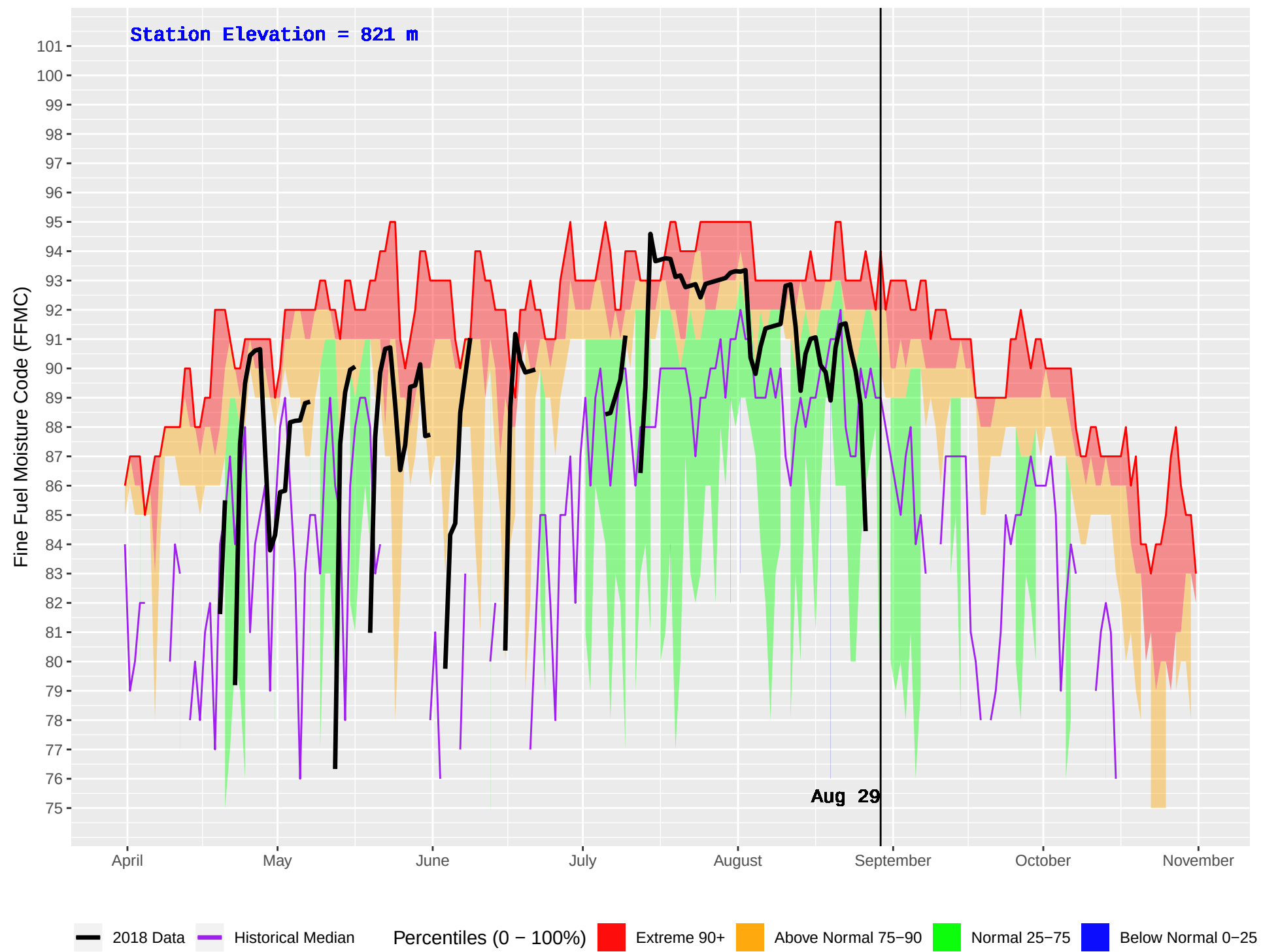
AKOKLI CREEK (838) : Historical (2003–2016) and Current (2018) Daily Fine Fuel Moisture Code (FFMC)
